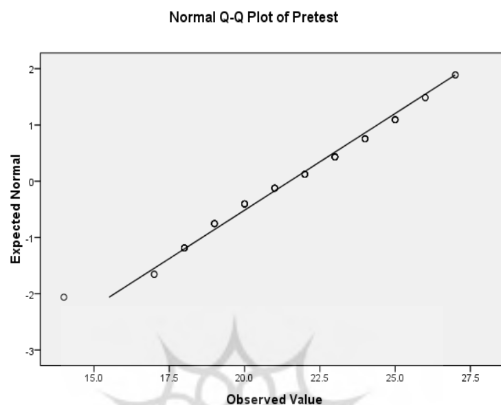
Fig. 1. Normal Q-Q Plot of Pre-test
