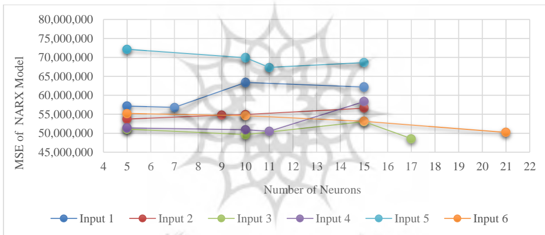
Figure (4) Sensitivity analysis of the NARX model to the number of neurons
