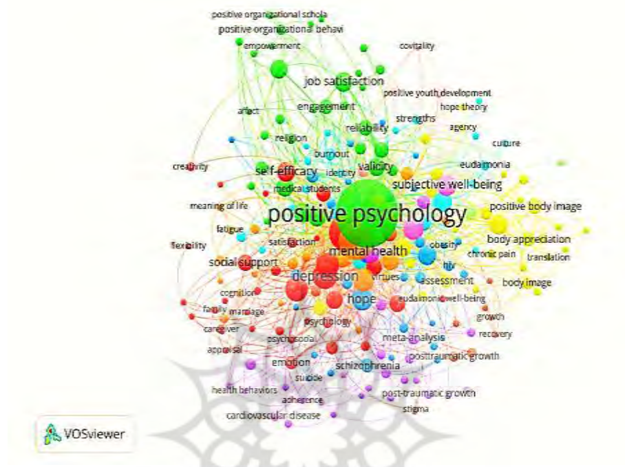
Figure 1. Co-occurrence network of keywords by authors
