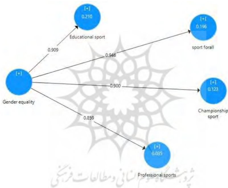
Figure 1. Structural model of research with path coefficients
