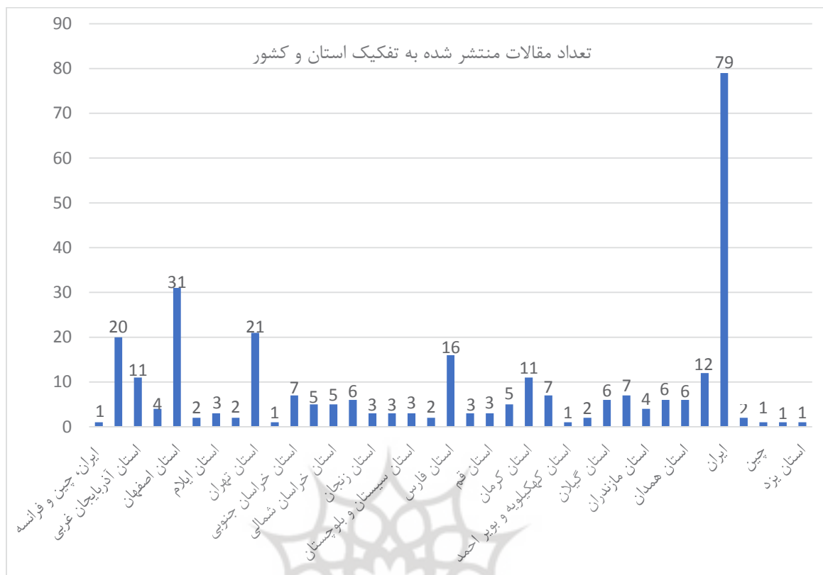
Graph. 2: Articles Published in the Province or Country Under Study (Authors, 2024).
