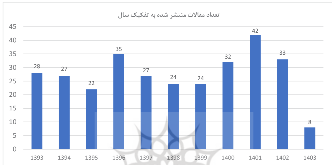
Graph. 1: The number of articles published annually, categorized by year, from 2014 to 2024 (Solar Hijri calendar: 1393–1403). (Authors, 2024).
