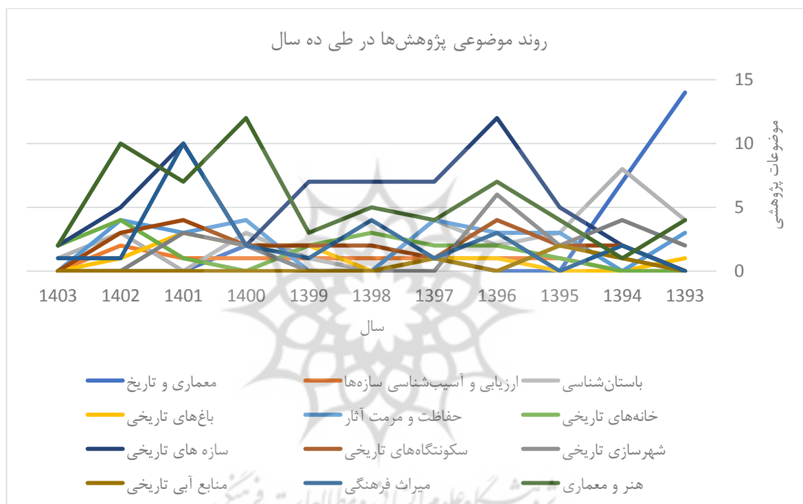
Graph. 5: Thematic Trends of Research over a 10-Year Period (Authors, 2024).
