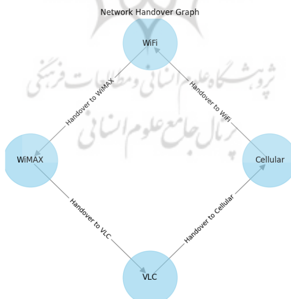
Figure 3. Implementation Scenario
