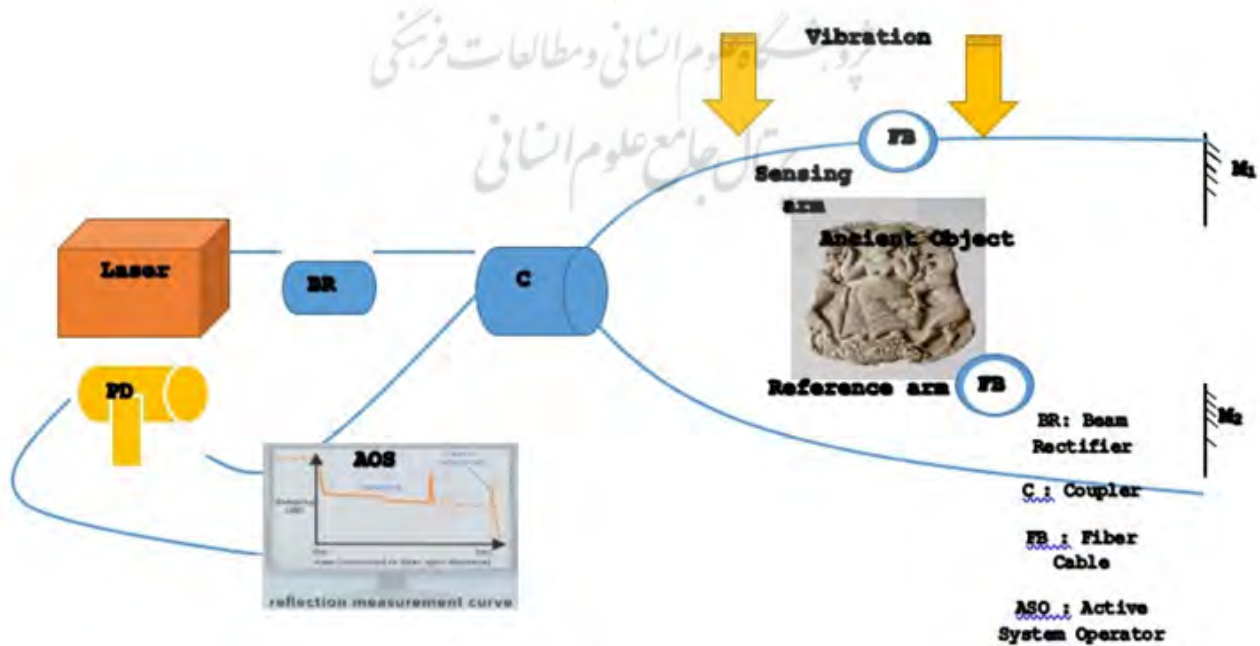
Fig 8. Simple schematic of a fiber optic protection system protecting an ancient specimen using Michelson interferometry.
