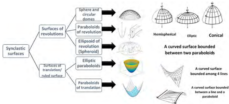
Fig. 6: Typology of synclastic gridshells based on their geometries (Source: Authors).
