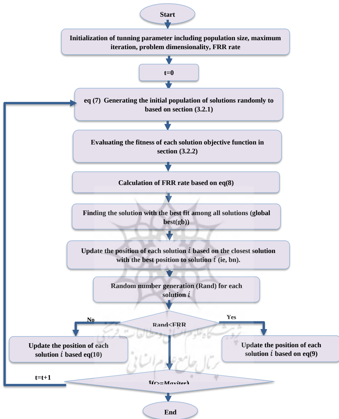
Fig. 3: Lemur optimization process based on neural network objective in the proposed method
