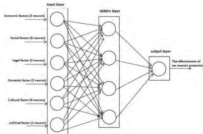
Fig. 2: Overall framework for predicting tax evasion using a perceptron neural network.
