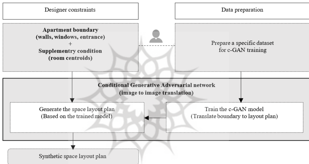
Fig. 3: Research methodology flowchart (Source:Authors)
