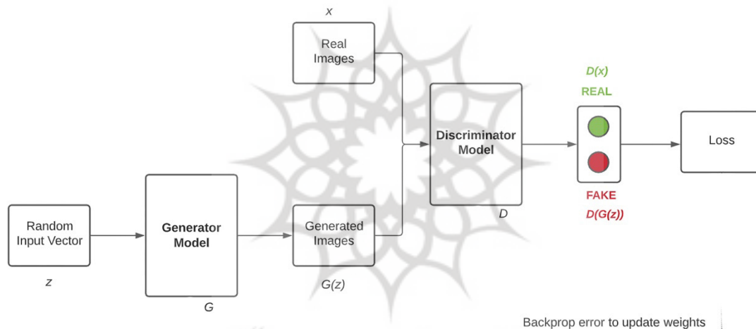
Fig. 4: The structure of Conditional GAN (Source:Authors)
