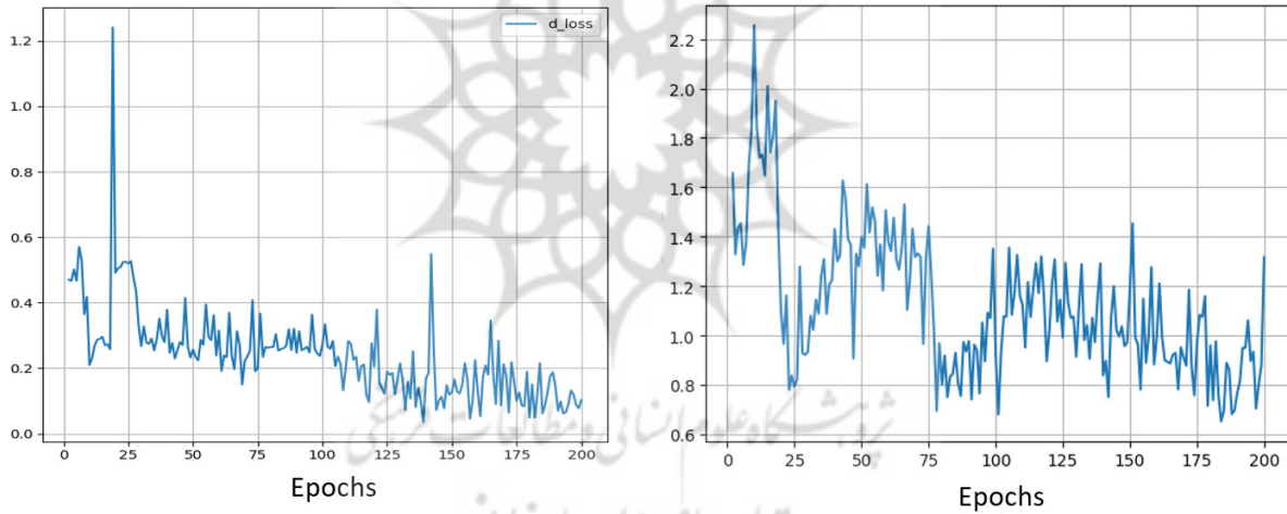
Fig.9: Discriminator loss (left), Generator loss (Right)
