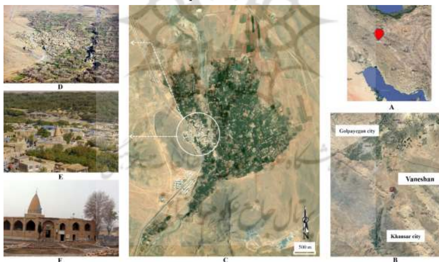
Fig. 1. A. Location of Vaneshan village in the country. B. The geographic position of Vaneshan between Khansar and Golpayegan city. C. Aerial photo of the village. (Behrah, 2024) D. the residential area in the center of farms. E & F. Abu- Al- Fotuh holy shrine
