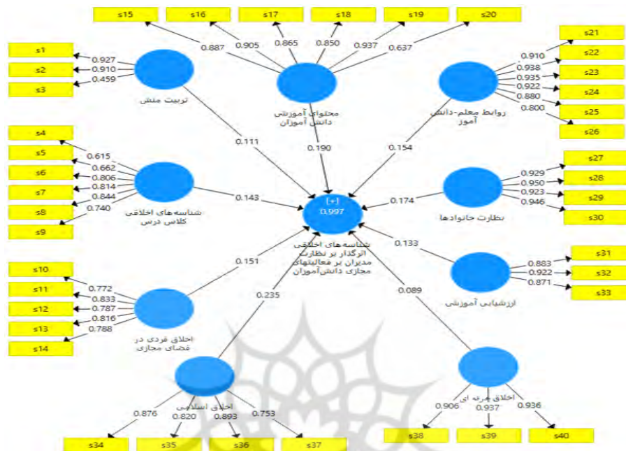
Figure 2. Standard path coefficients of the research model
