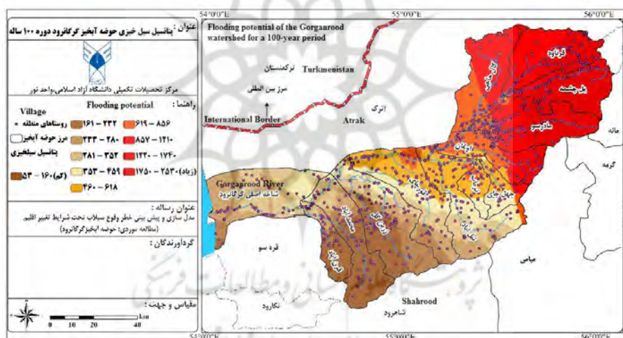
Fig.6. Zoning of future flood risk using the output of SWAT method for 50 years period
