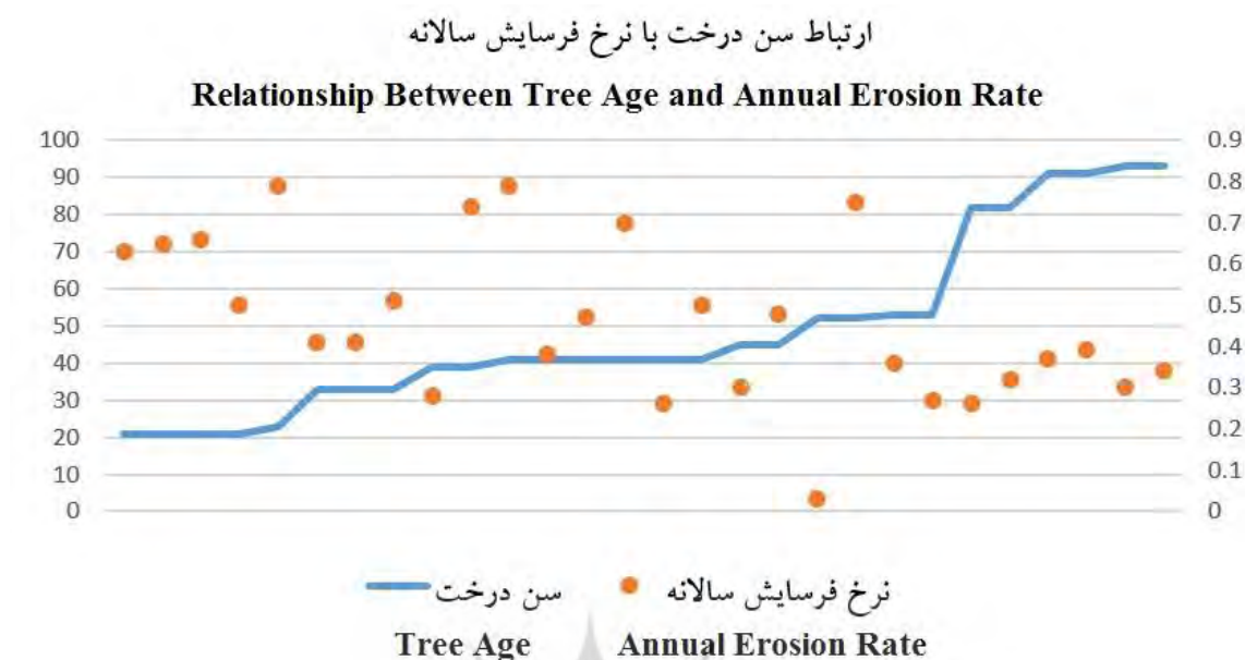
Fig.7. Relationship Between the Age of Sampled Trees and the Annual Erosion Rate
