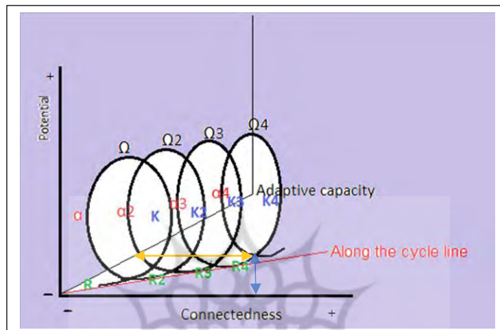
Figure 3. Adaptive groundwater cycle concerning resilience line and connectedness
